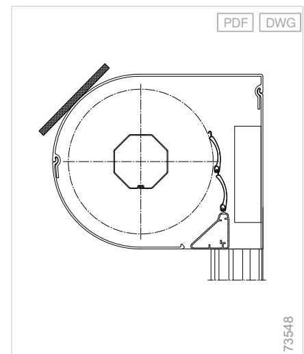
Vorbau-Rollladen V10, Rund, EWFS SolarKit
